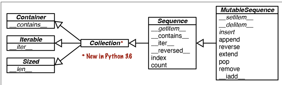
Figure 13-3. UML class diagram for the MutableSequence ABC and its superclasses from collections.abc (inheritance arrows point from subclasses to ancestors; names in italics are abstract classes and abstract methods).
