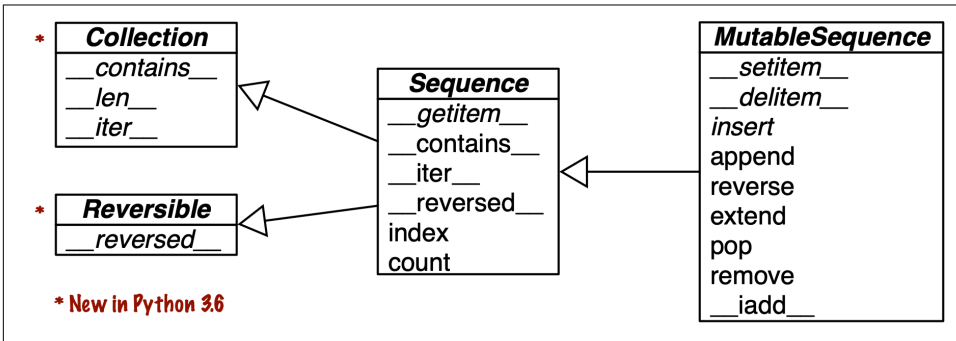
Figure 2-2. Simplified UML class diagram for some classes from collections.abc (super-classes are on the left; inheritance arrows point from subclasses to superclasses; names in italic are abstract classes and abstract methods).
